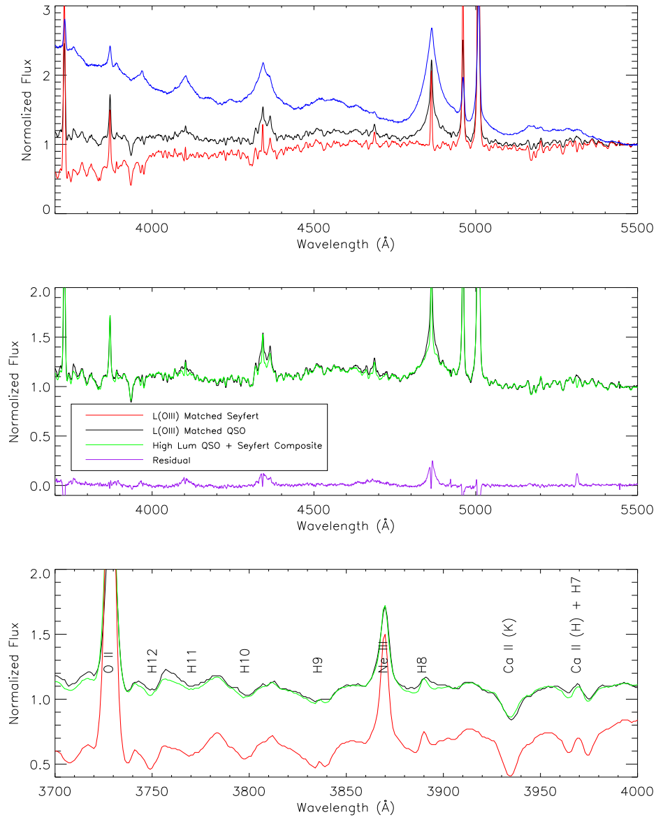
Figure 22: Top: The composite type 2 AGN spectrum is shown in red. The composite spectrum of matched QSOs is shown in black. A composite spectrum of QSOs with very high continuum luminosities is shown in blue. Middle: A linear combination of 70 % type 2 AGN + 30 % pure QSO (green ) is compared to the matched QSO spectrum (black). The residual is shown in purple. Bottom: The spectral region between 3700 and 4000 Å is shown in more detail. The main stellar absorption lines, including the higher-order Balmer lines and Calcium H+K lines have been marked for clarity.
